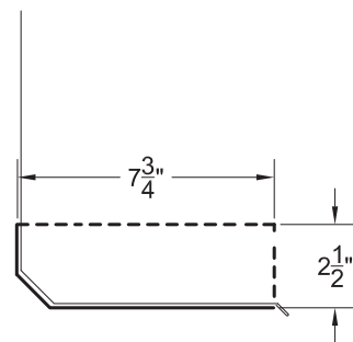
END DAM PROFILE NOTE: All dimensions to be field verified prior to fabrication
